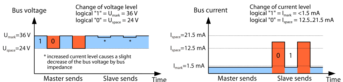
Figure 6: Signalling on the M-Bus
