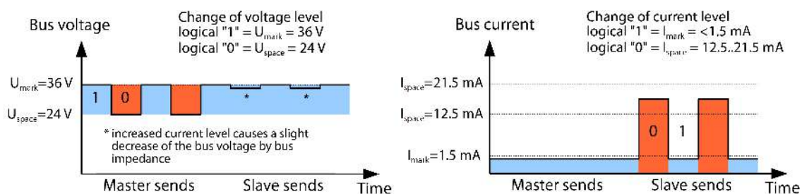
Figure 31: Signalling on the M-Bus
