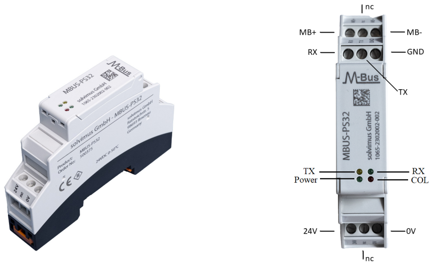
Figure 1: MBUS-PS32, view (left), connectors and LEDs (right)
