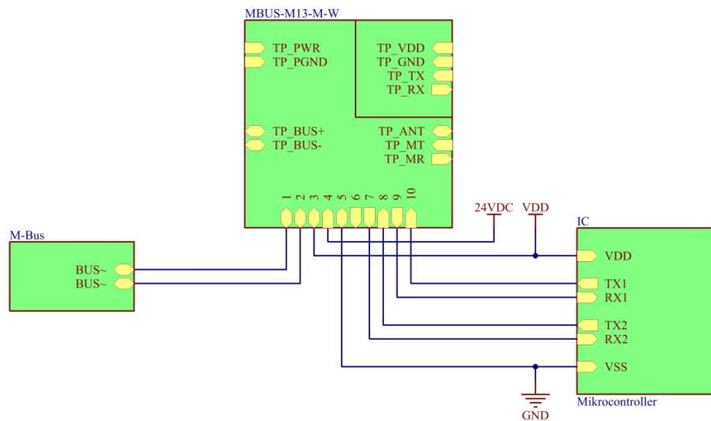
Figure 2: MBUS-M13-M-W with exclusive use of the X1 connector
