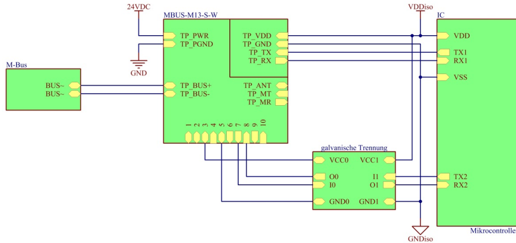
Figure 1: MBUS-M13-S-W with galvanically isolated logic interface
