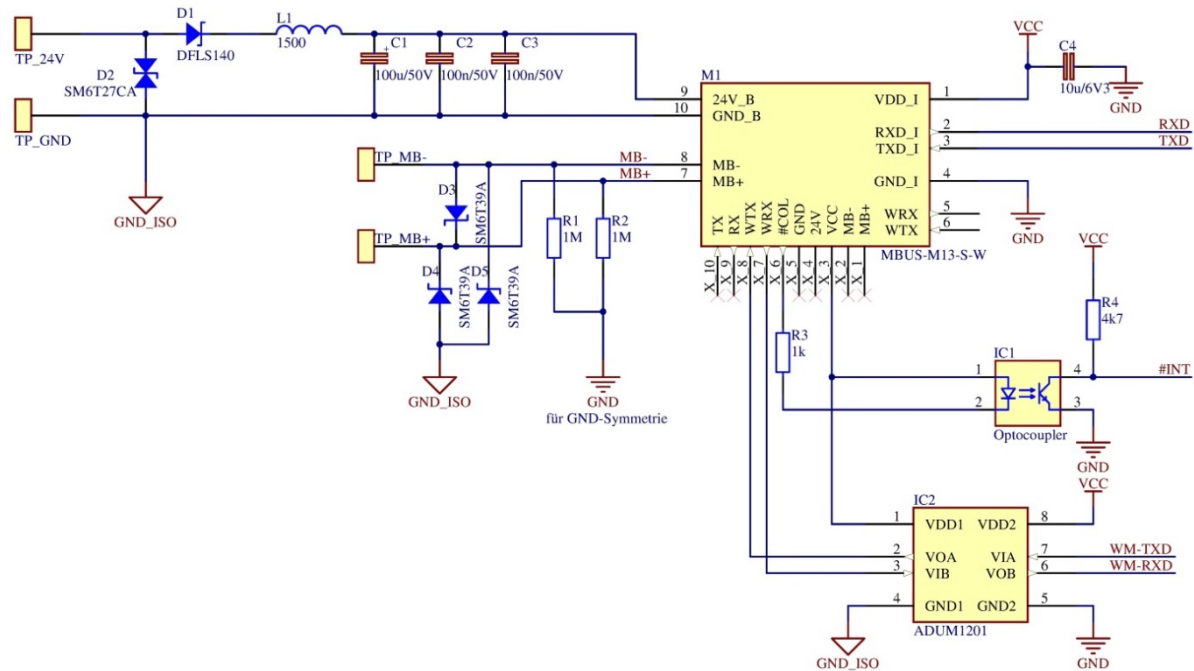
Figure 3: Reference circuit for the MBUS-M13-S-W
