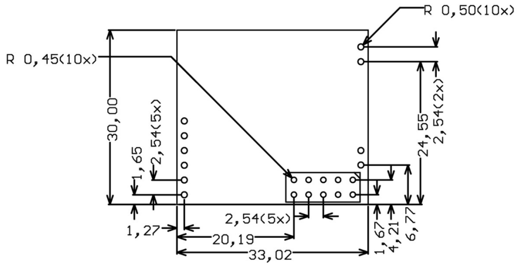
Figure 3: Mechanical dimensions and position of pads of MBUS-M13 (values are in mm)
